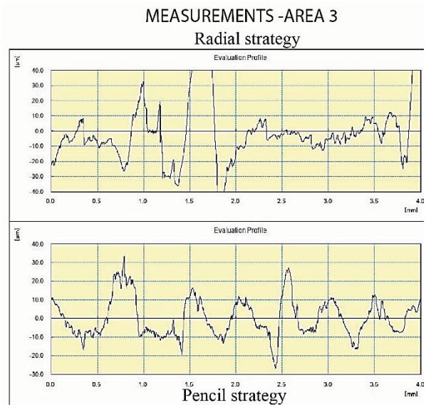
Figure 18: Roughness profile in area 3 in horizontal direction for radial and pencil strategies
